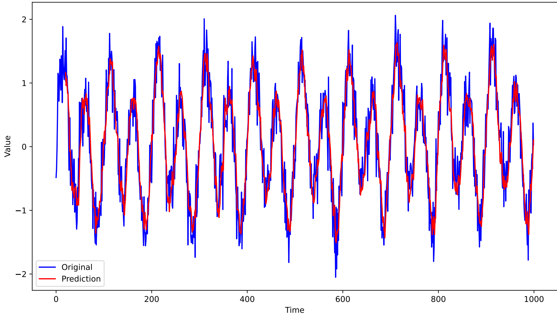
Greedy sparse AR(20) LS one step prediction
